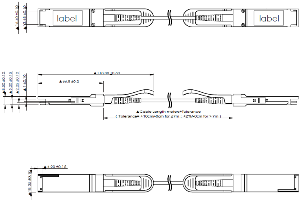
Figure 3 –Mechanical Dimensions
