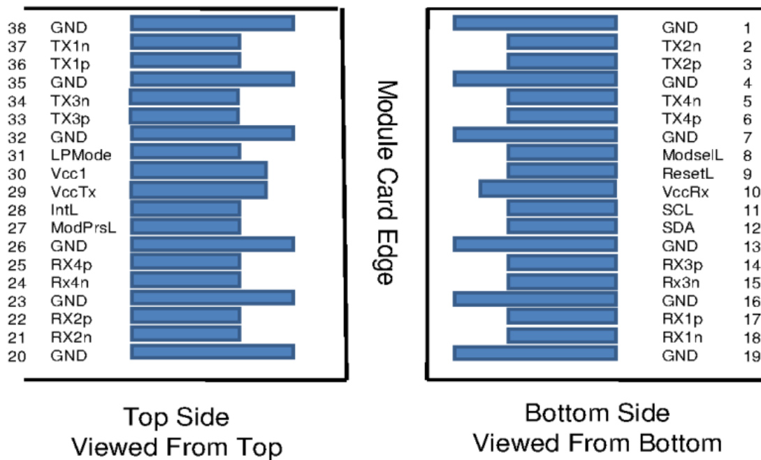
Figure 1 – Pin Definitions
