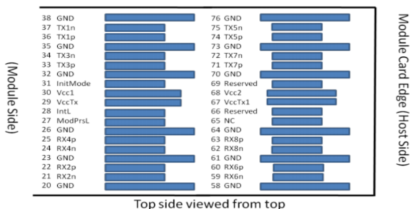
Legacy QSFP28 Pads
